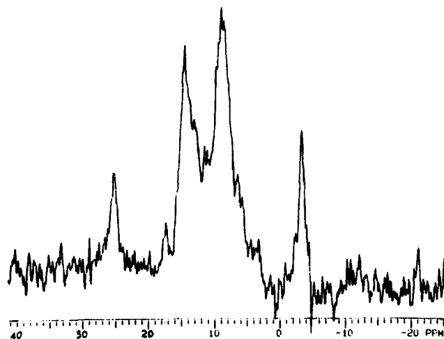
Figure 3. Low-temperature ^{29}\text{Si} NMR spectrum of polymer 1 ( \text{X} = \text{O} ).
